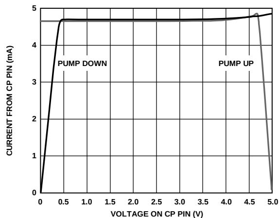
Figure 10. Charge Pump Characteristics at CP_V = 5.0 V
