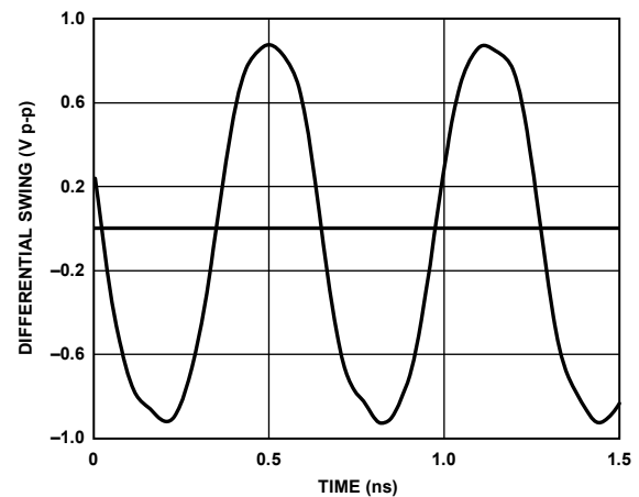
Figure 17. LVPECL Differential Voltage Swing at 1600 MHz
