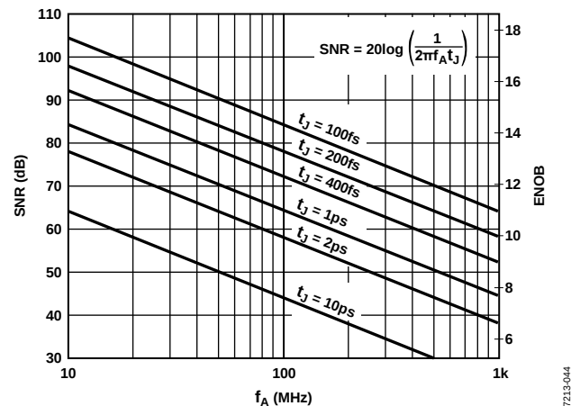
Figure 70. SNR and ENOB vs. Analog Input Frequency
