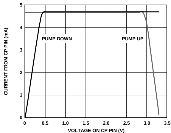
Figure 9. Charge Pump Characteristics at CP_V = 3.3 V
