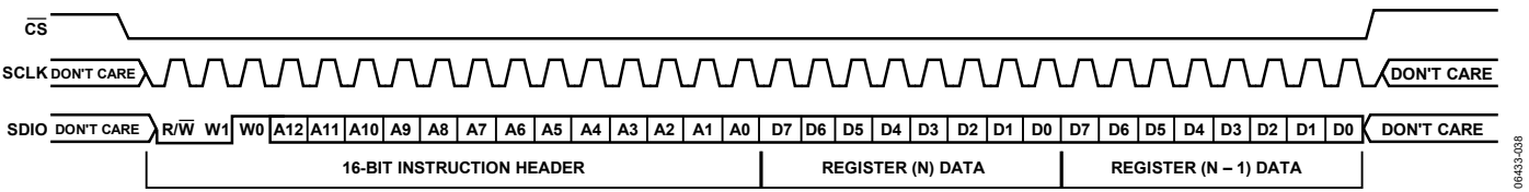
Figure 46. Serial Control Port Write—MSB First, 16-Bit Instruction, Two Bytes Data
