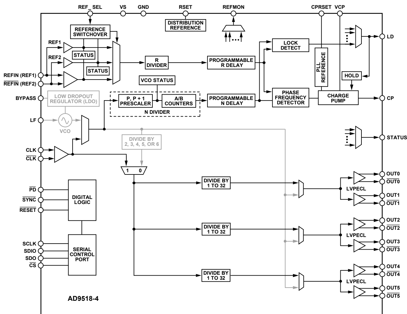
Figure 30. Clock Distribution or External VCO < 1600 MHz
