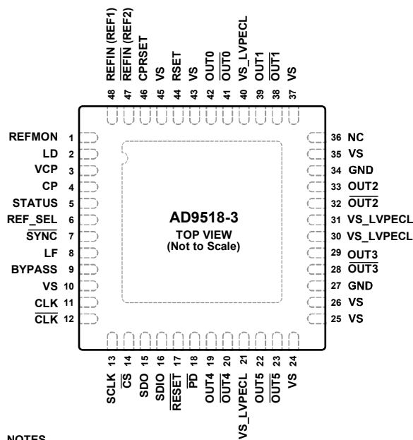
Figure 4. Pin Configuration
