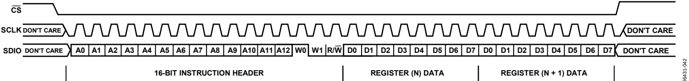
Figure 50. Serial Control Port Write—LSB First, 16-Bit Instruction, Two Bytes Data
