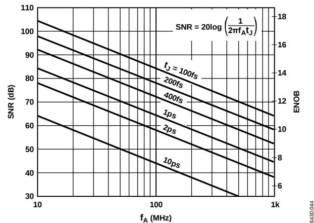
Figure 52. SNR and ENOB vs. Analog Input Frequency
