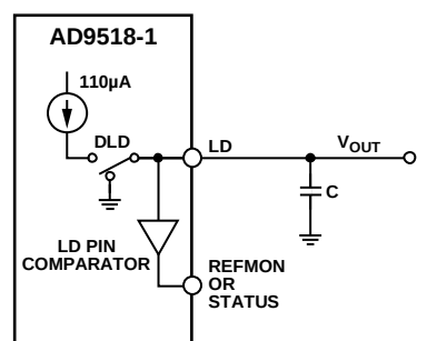
Figure 36. Current Source Digital Lock Detect
