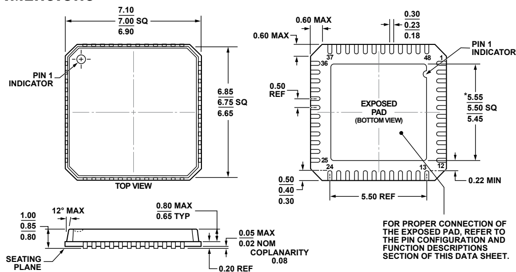
Figure 56. 48-Lead Lead Frame Chip Scale Package [LFCSP_VQ] 7 mm x 7 mm Body, Very Thin Quad (CP-48-8) Dimensions shown in millimeters
