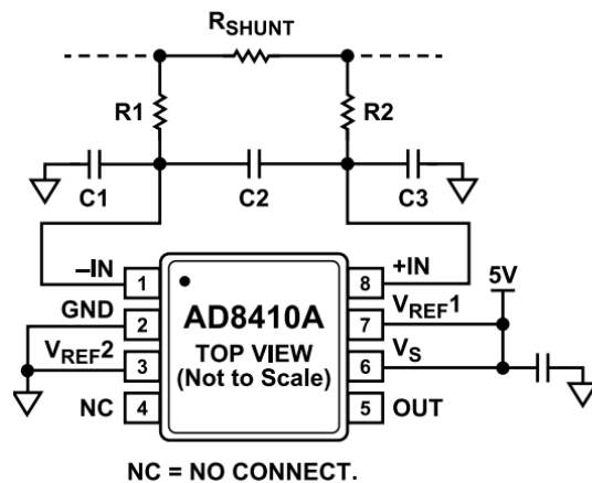
Figure 64. Input Filter
