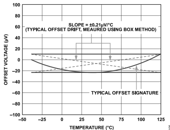
Figure 57. Box Method
