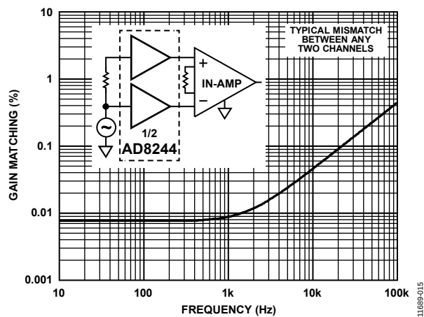
Figure 15. Gain Matching vs. Frequency, 1 k \Omega Source Imbalance
