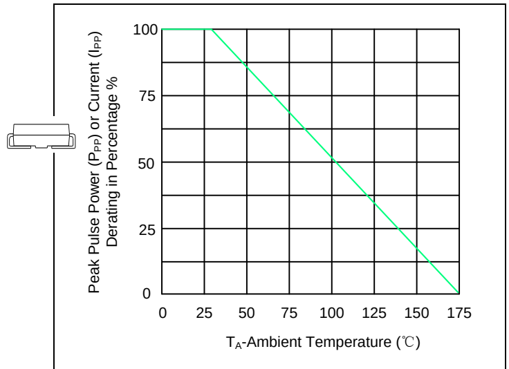
Figure 2. Pulse Derating Curve
