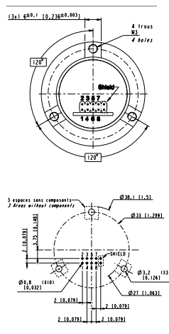
RJF TV6A 7S X 5 X F059 Receptacle CAT6A
