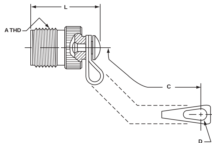
PLUG PROTECTION CAP MS25042-XXDA*
