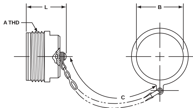
PLUG PROTECTION CAP 10-329391-XX*
