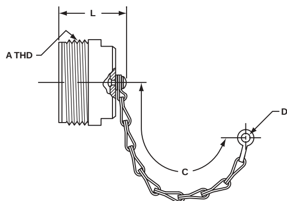
PLUG PROTECTION CAP MS25042-XXDA*
