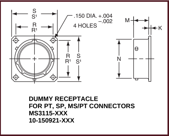
DUMMY RECEPTACLES – FOR PT, SP, MS/PT
