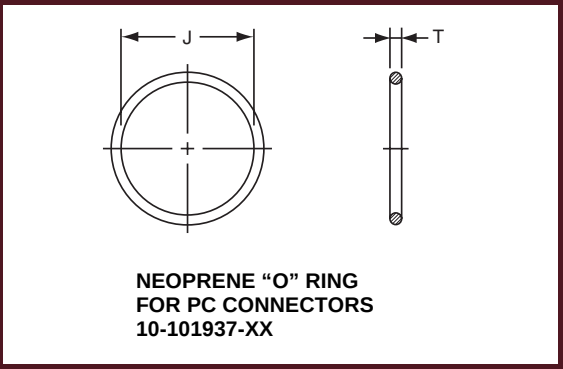
NEOPRENE “O” RINGS – FOR PC
