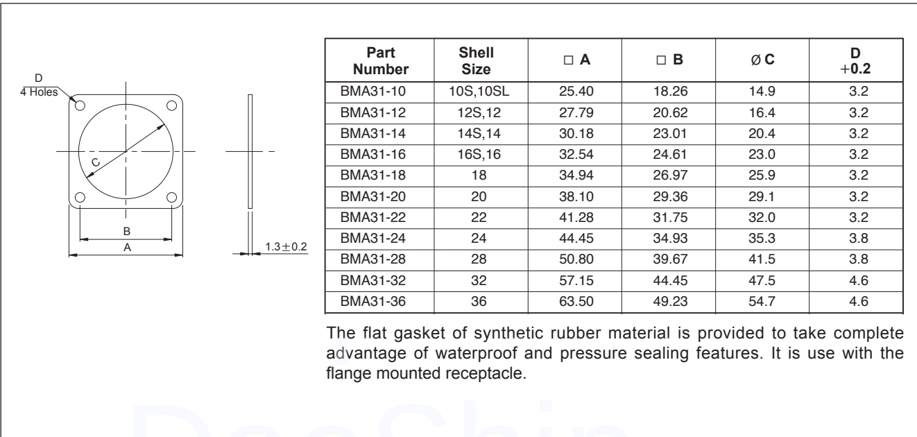
Sealing Gasket BMA 31
