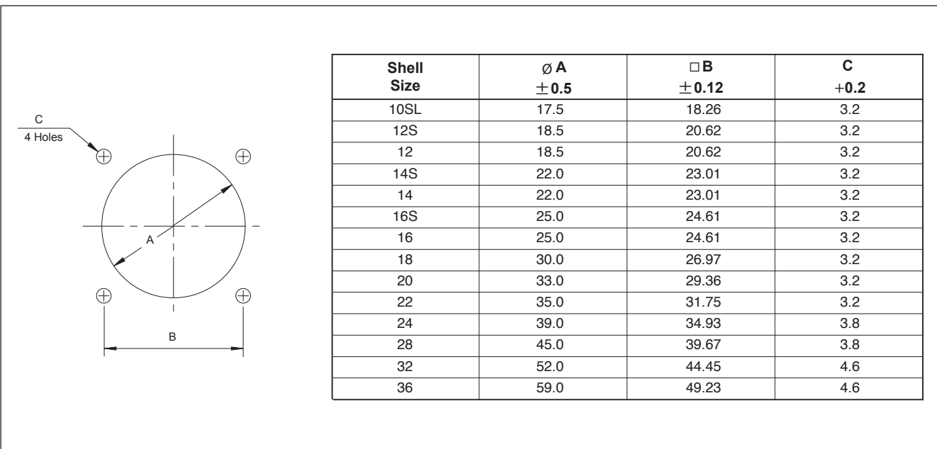
Panel Mounting Hole(Reference)
