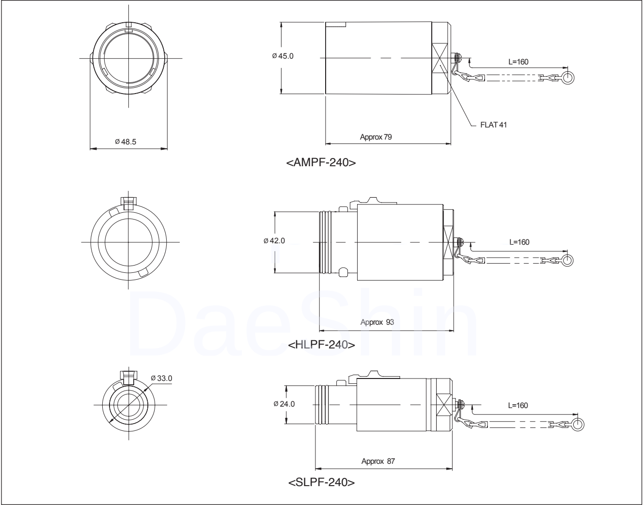
Receptacle Protection Cap (mm)
