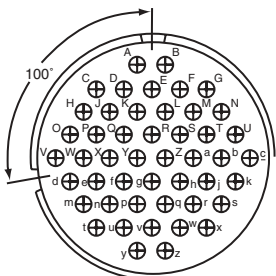
100° Rotation of 36-10
