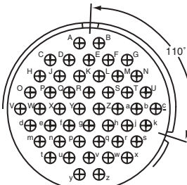
110° Rotation of 36-10
