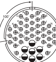
100° Rotation of 36-7
