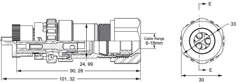
C10-730513-Z3S 3 WAY 400VDC/250V AC STRAIGHT PLUG IEC61984 & IEC60950-22 Certified
