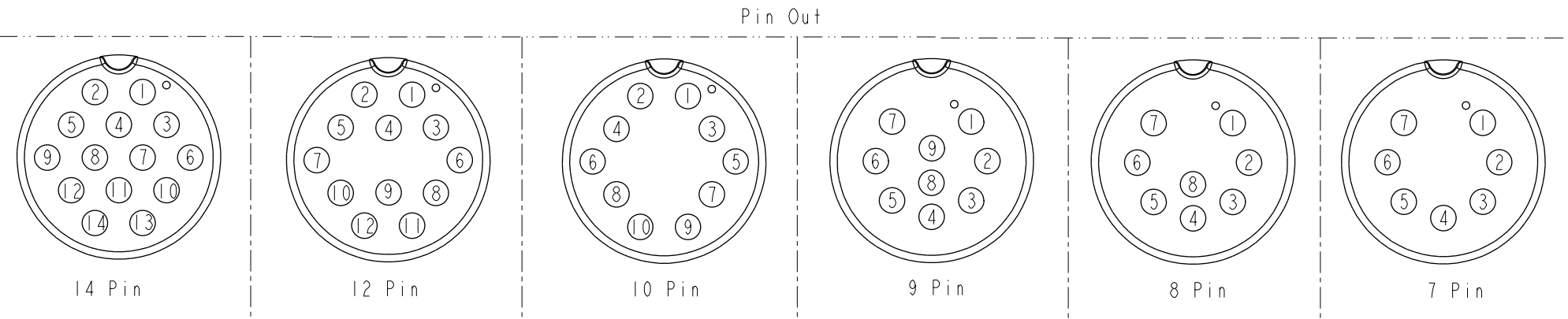
Pin Assignments Front View
