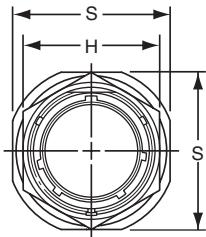
TERMINATION ASSEMBLIES "CE" (SR) Strain Relief
