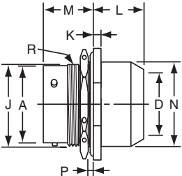
PT07CP-XX-XX SP07CP-XX-XXX
