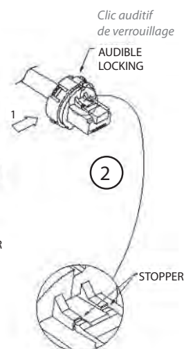
HALF INSULATOR Demi-isolant
