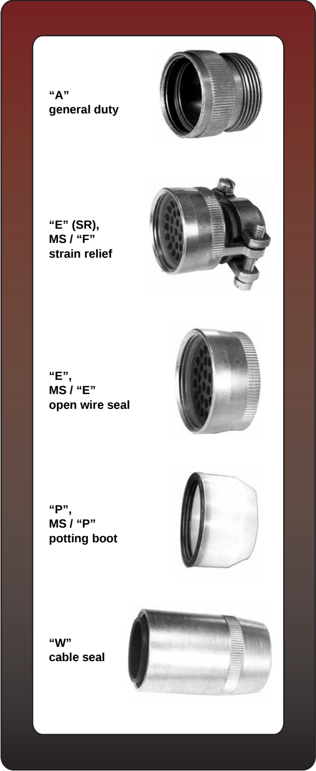
BAYONET COUPLING WITH SOLDER CONTACTS PT, SP, MS/PT
