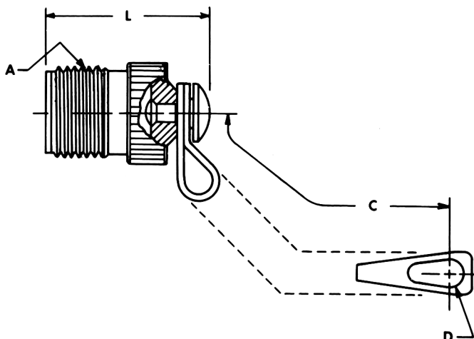
PLUG PROTECTION CAP MS25042-XXDA*
