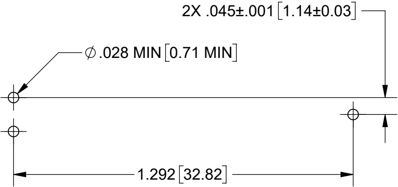
RECOMMENDED MOUNTING HOLE PATTERN
