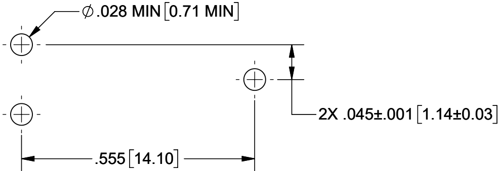
RECOMMENDED MOUNTING HOLE PATTERN
