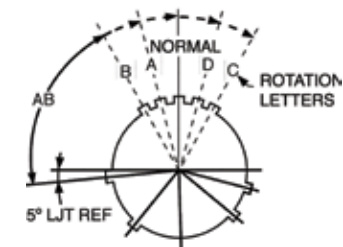
RELATIVE POSSIBLE POSITION OF ROTATED MASTER KEYWAY (front face of receptacle shown)
