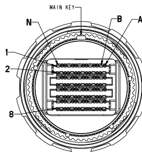
Wiring Table Size 23 and 25 Tx: Rx Signal Map
