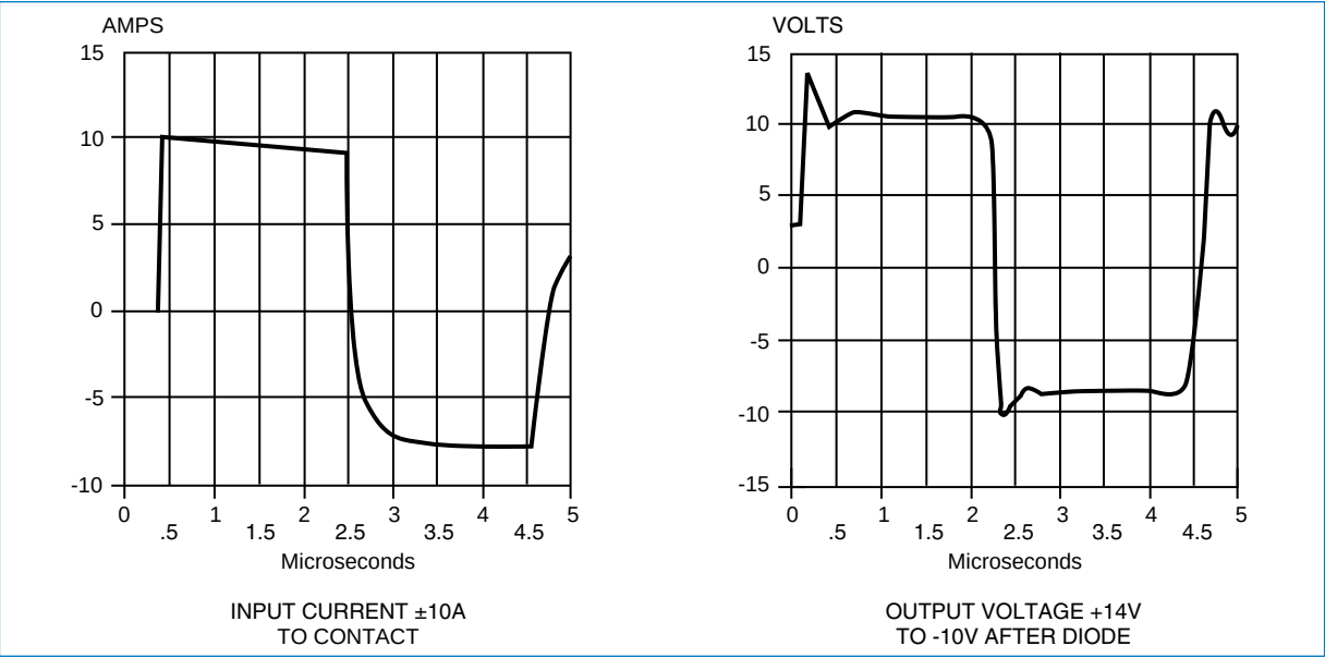
DIODE CONTACT PULSE TEST, ±5.8 DIODE
