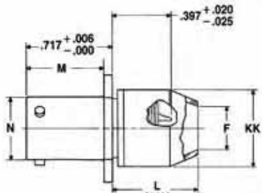
LJT01P-XX-XXX
