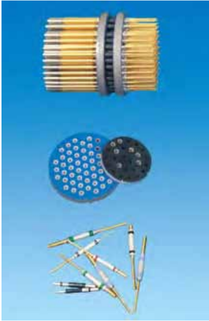
Planar Array Assembly
