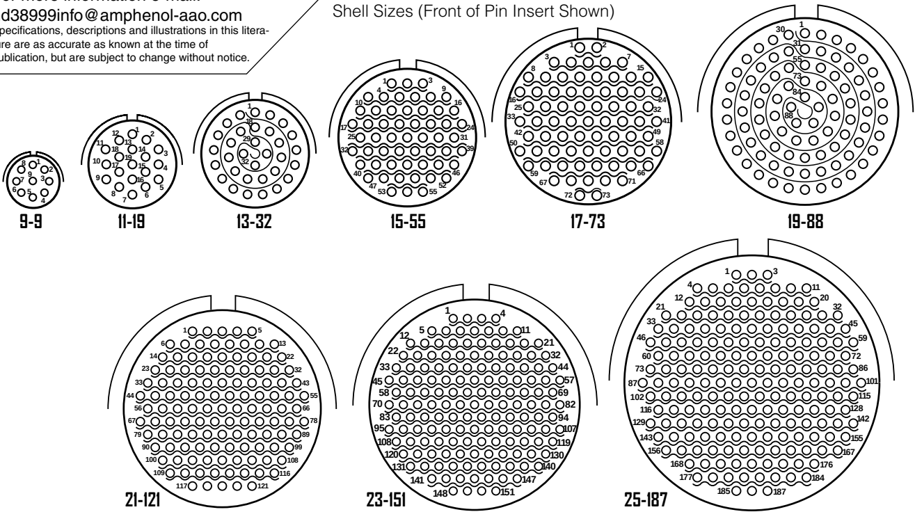
Shell Sizes (Front of Pin Insert Shown)
