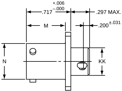
LJT02RE-XX-XXX (MS27496E)
