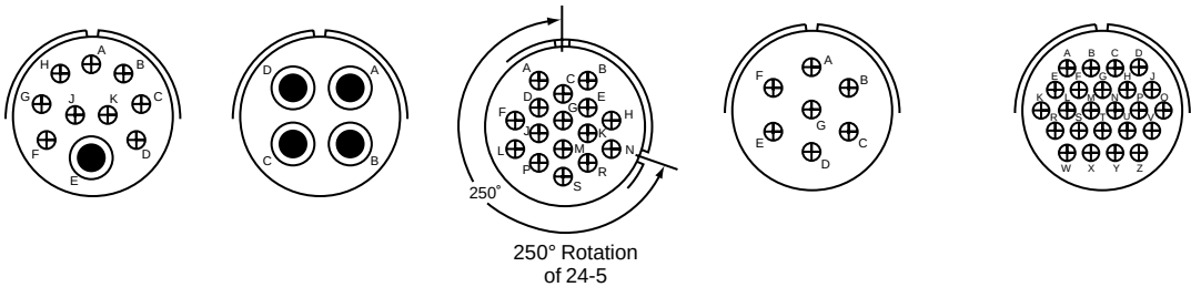
Front Face of Pin Insert or Rear Face of Socket Insert Illustrated
