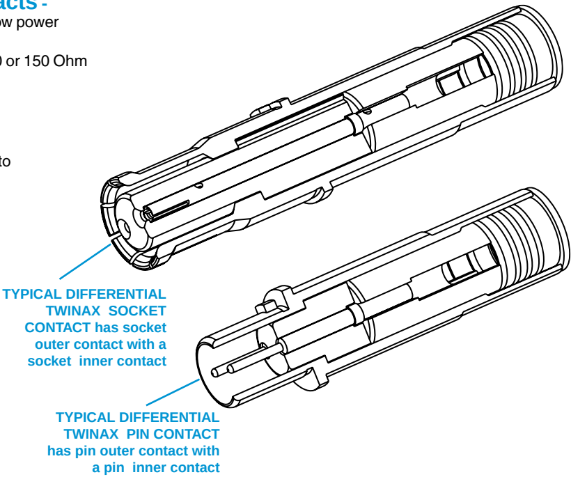
Cable Illustration - Differential Twinax Contact
