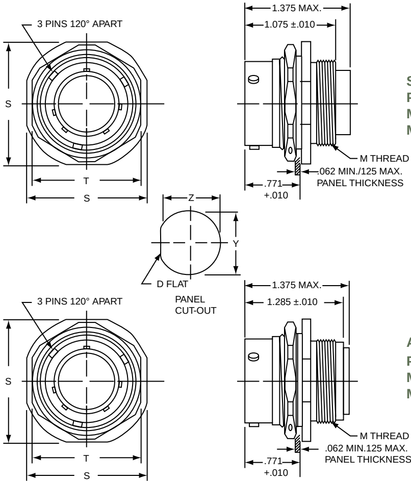
STAINLESS STEEL Pyle ZZW-RX-15XX Series MS24265EXXBXX Military Class E
