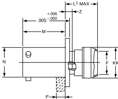
LJTPQ00RP-XX-XXX (MS27656P)
