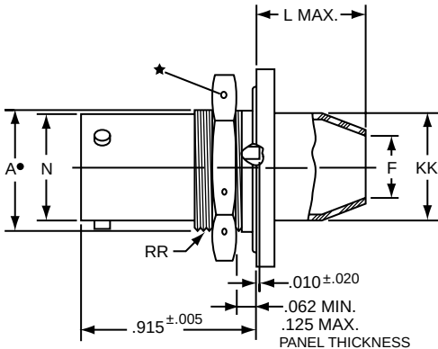
LJT07RP-XX-XXX (MS27468P)
