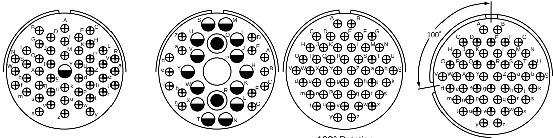
100° Rotation of 36-10
