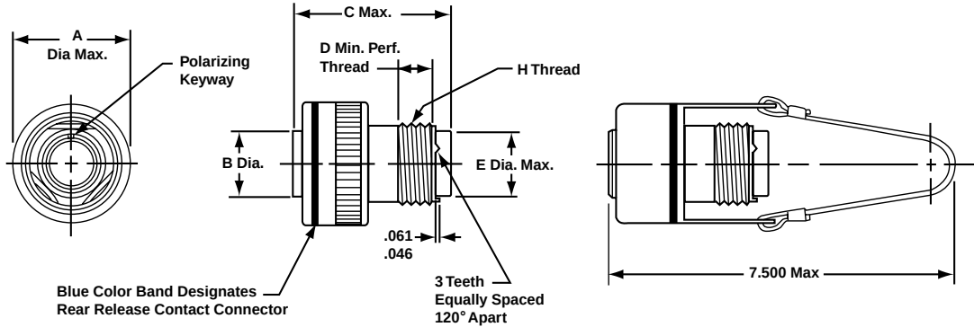
9818 Connector
