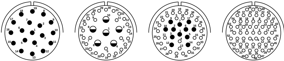
Front Face of Pin Insert or Rear Face of Socket Insert Illustrated
