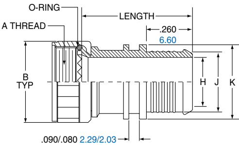
STRAIGHT ENTRY ROTATABLE COUPLING 2M440MS135
