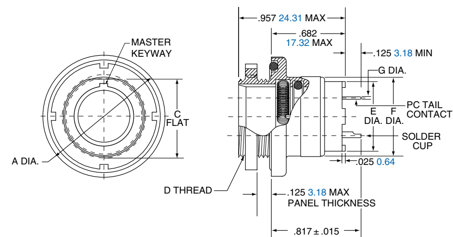
2M804-006-07
