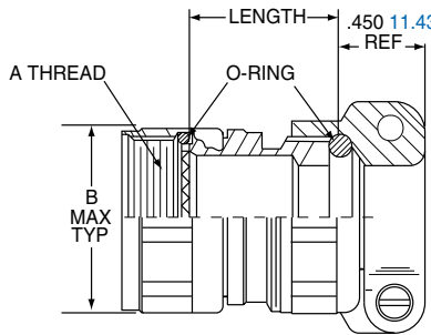
45° ENTRY ROTATABLE COUPLING 2M370MB038
