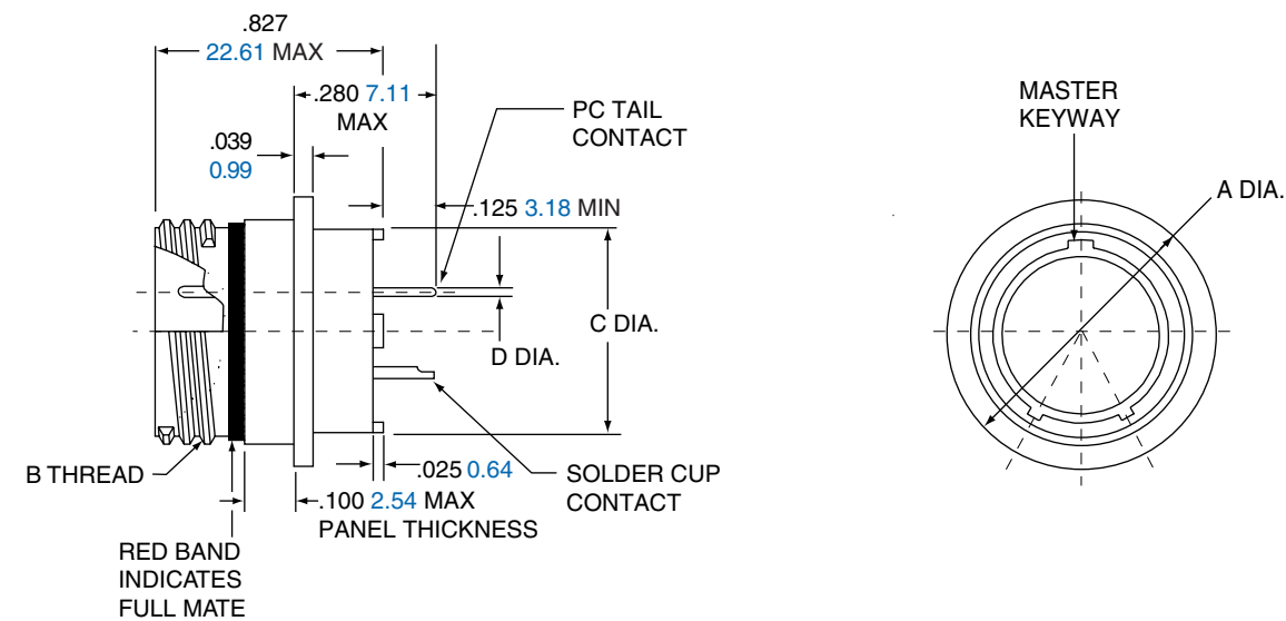
2M805-006-03
