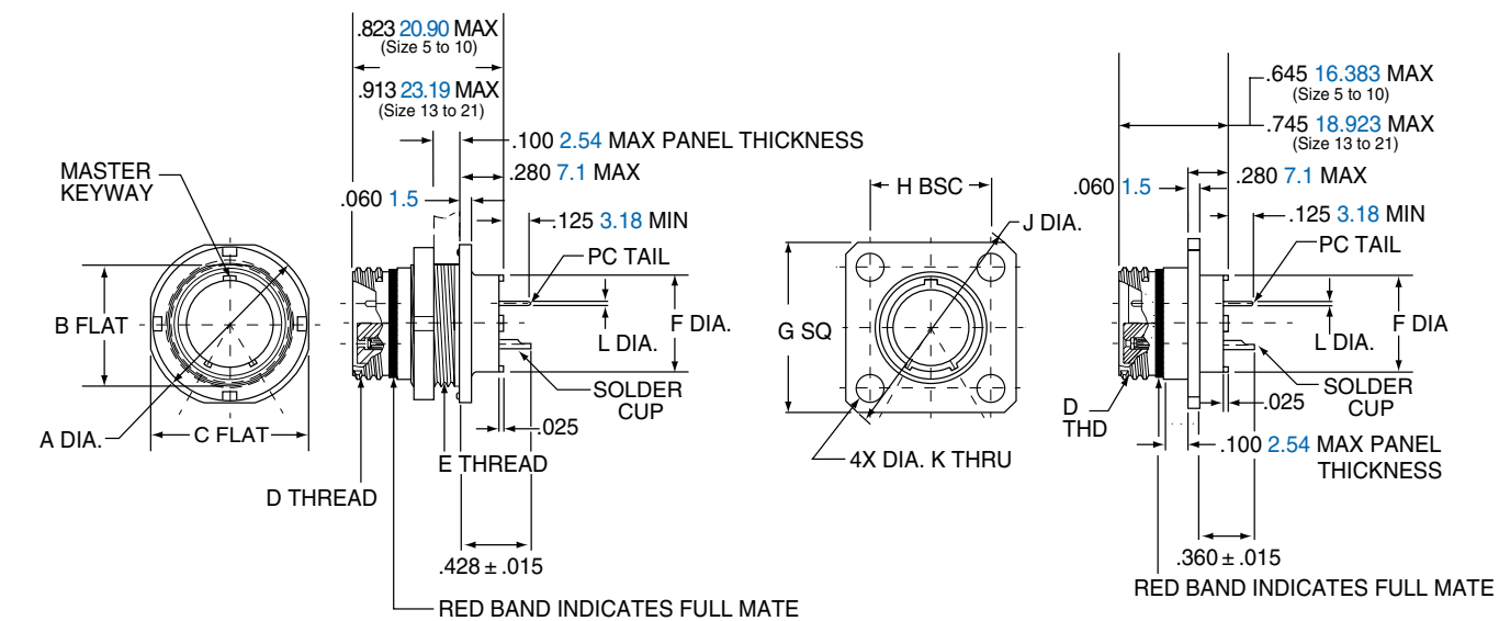
2M801-011-07 2M801-033-07
