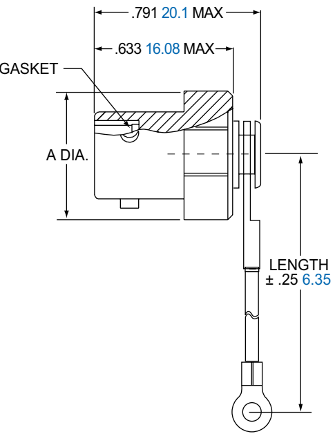
2M660-082
