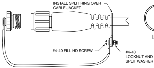
Large Split Ring designed for attaching covers to cables
