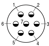
Front face of pin inserts illustrated (Socket Reversed)
