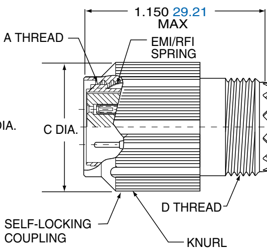
2M805-002
