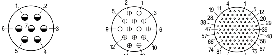
Front face of pin inserts illustrated (Socket Reversed)
