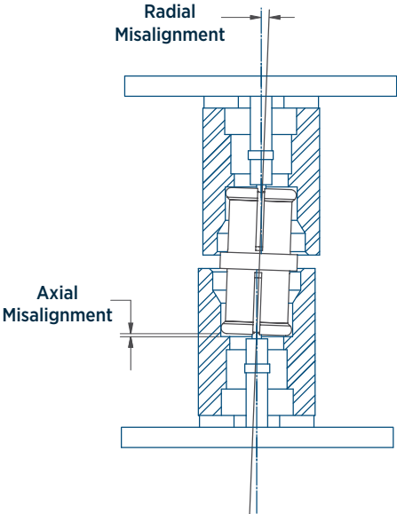
Figure 3: Radial and Axial Misalignment Definitions
