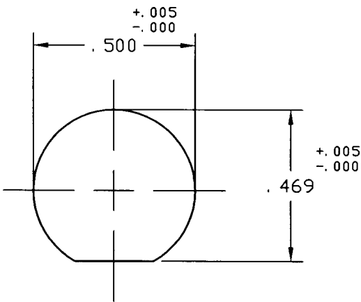
RECOMMENDED MTG. HOLE DETAIL (MAX PANEL THK. .115)
