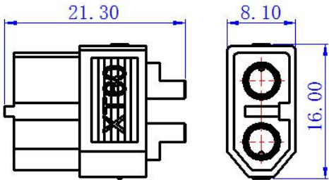
XT60-F
