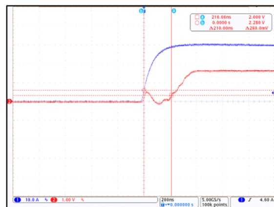
Figure 10: CT431 Propagation Delay; I_P = 30\text{ A}_{PK} and C_L = 100\text{ pF} (Blue = I_{CCC} , Red = V_{OUT} )
