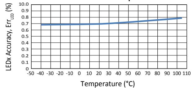
LED Set Point Accuracy versus Ambient Temperature
