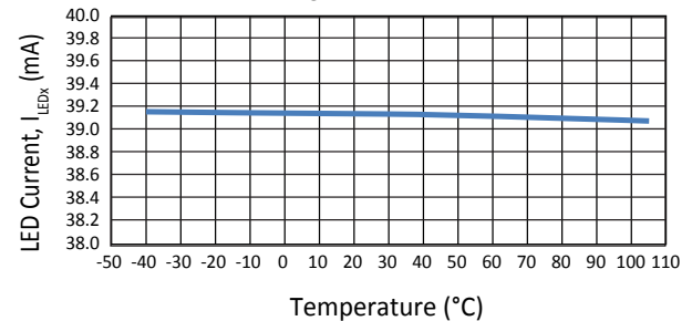
LEDx Current versus Ambient Temperature I SET = 120 μA
