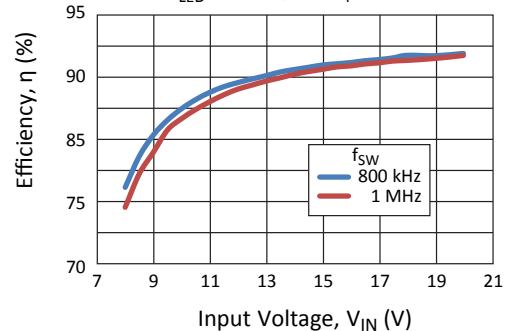
Efficiency for 12 Series LEDs per Channel I LED = 40 mA, LED V f ≈ 3.2 V
