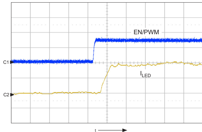
Figure 12C. Delay from rising edge of PWM signal to LED current; shows EN/PWM (ch1, 2 V/div.), and I_{LED} (ch2, 20 mA/div.), t = 200 ns/div.
