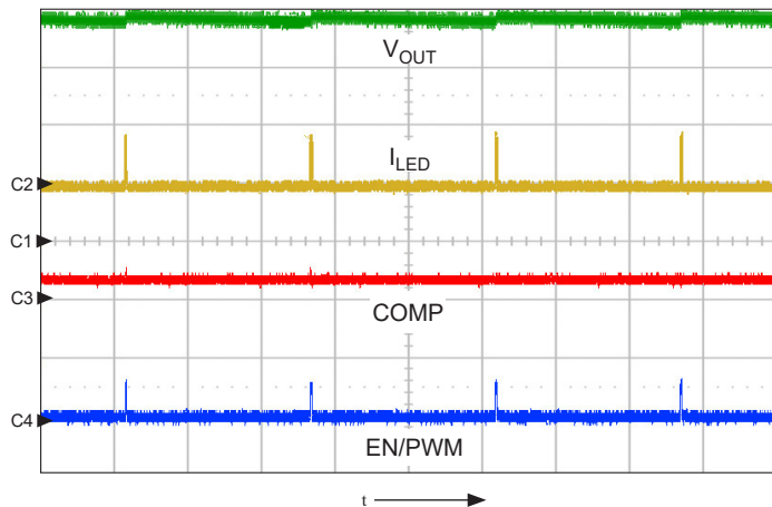
Figure 12B. Typical PWM diagram showing V_{OUT} , I_{LED} , and COMP pin as well as the PWM signal. PWM dimming frequency is 200 Hz at 1% duty cycle ; shows V_{OUT} (ch1, 10 V/div.), I_{LED} (ch2, 50 mA/div.), COMP (ch3, 2 V/div.), EN/PWM (ch4, 5 V/div.), t = 2 ms/div.
