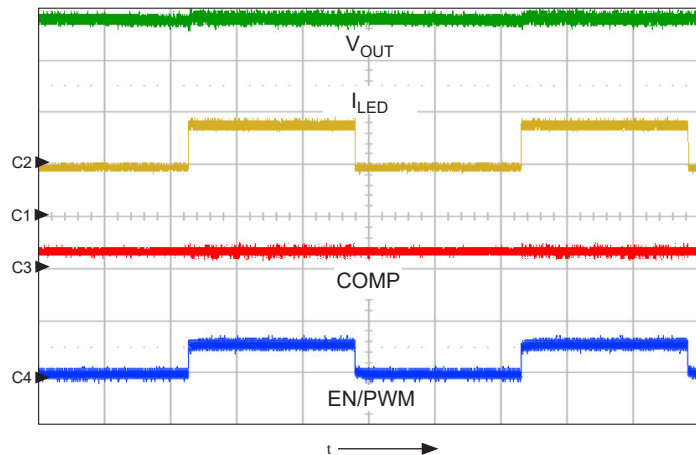
Figure 12A. Typical PWM diagram showing V_{OUT} , I_{LED} , and COMP pin as well as the PWM signal. PWM dimming frequency is 200 Hz at 50% duty cycle; shows V_{OUT} (ch1, 10 V/div.), I_{LED} (ch2, 50 mA/div.), COMP (ch3, 2 V/div.), EN/PWM (ch4, 5 V/div.), t = 1 ms/div.
