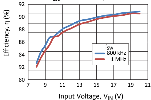
Efficiency for 10 Series LEDs per Channel I LED = 40 mA, LED V f ≈ 3.2 V
