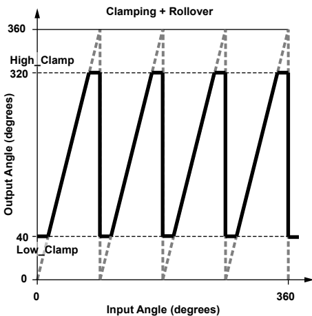
Figure 24: CE = 1, ROE = 1. Applied gain = 4x. LOW_CLAMP = 10 (≈40°), HIGH_CLAMP = 10 (≈320°)
