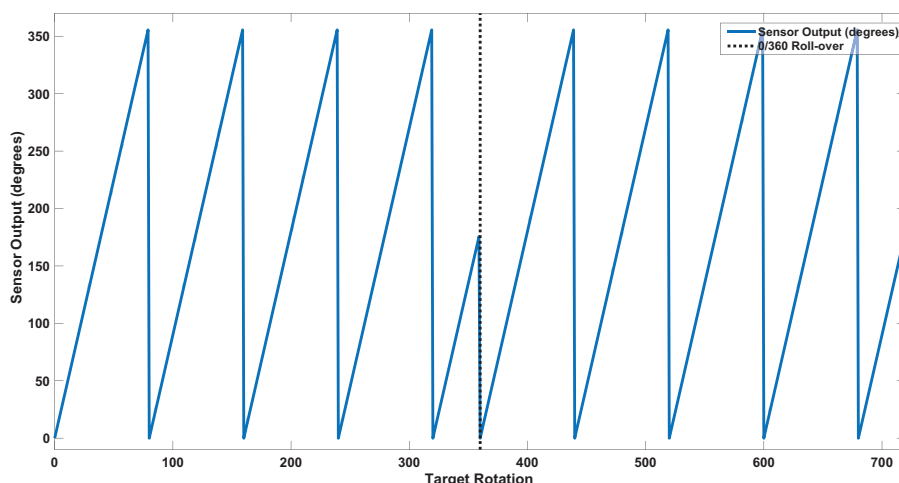
Figure 20: A1330 Output (in degrees) with 4.5× Gain
