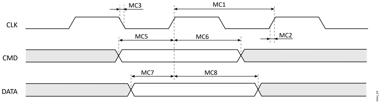
Figure 5-19 SDMMC Timing Diagram (SDR12/SDR25)
