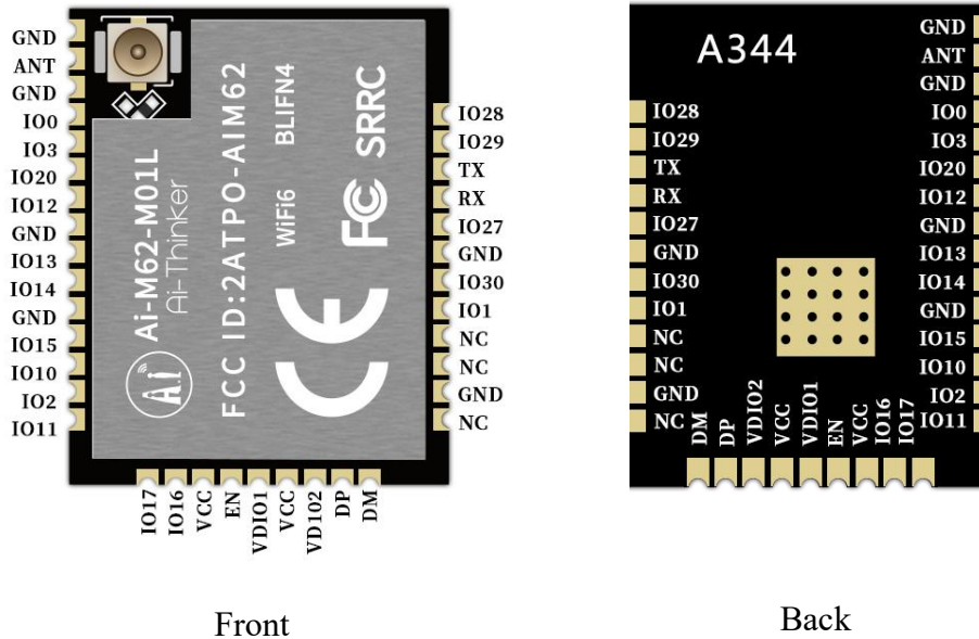
Figure 6 pin diagram
