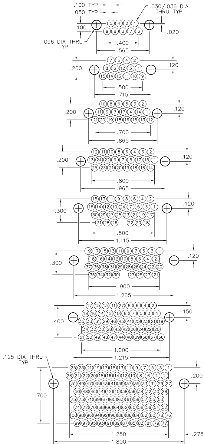
RECEPTACLE PC BOARD LAYOUT COMPONENT SIDE
