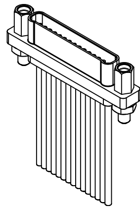
MM-122-015-261-22WQ (RECEPTACLE)
