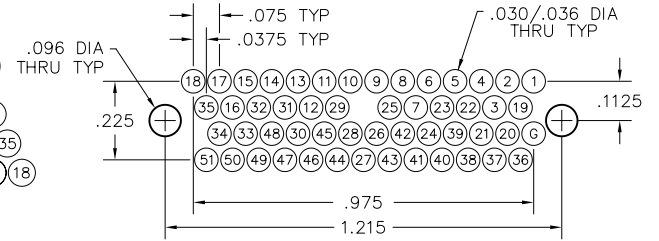
RECEPTACLE PC BOARD LAYOUT COMPONENT SIDE
