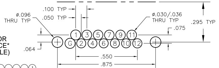
FRONT FACE OF FLANGE
