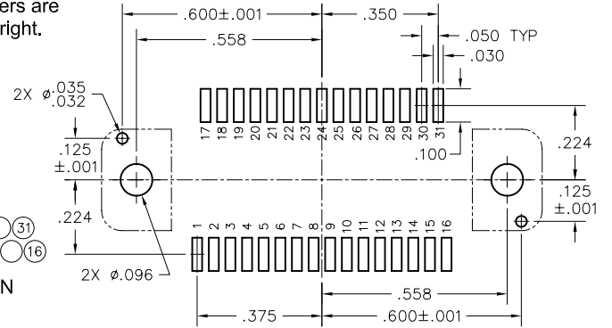
RECEPTACLE PC BOARD LAYOUT COMPONENT SIDE
