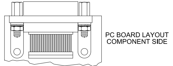
RECEPTACLE PC BOARD LAYOUT COMPONENT SIDE
