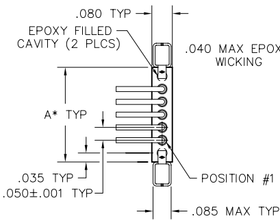
TERMINATION VIEW
