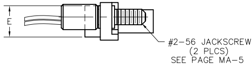
PLUG
