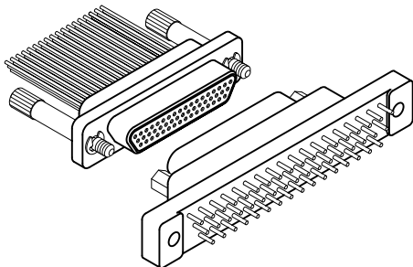
Rugged Straight, Narrow Footprint
