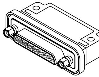
MK-2D2-031-335-260S (PLUG)
