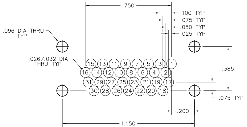
RECEPTACLE PC BOARD LAYOUT COMPONENT SIDE
