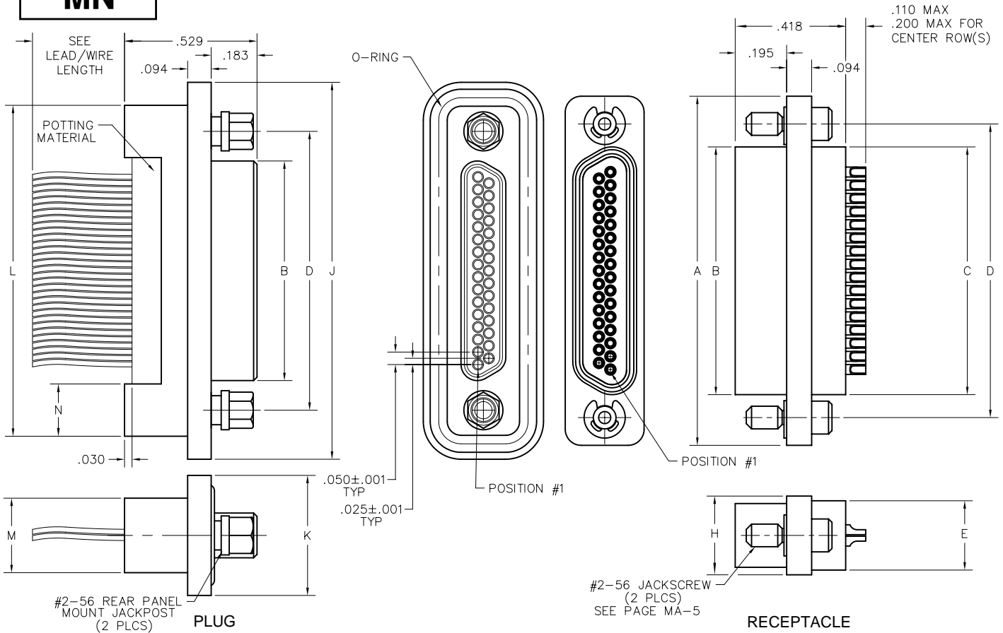
PLUG
