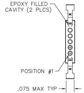
TERMINATION VIEW
