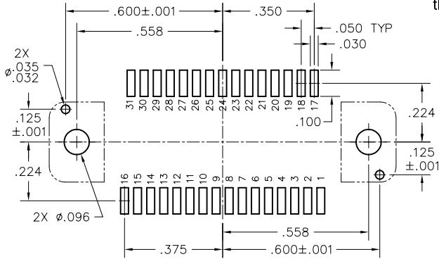
PLUG PC BOARD LAYOUT COMPONENT SIDE
