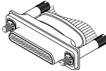
MM-2P2-031-161-44WA (PLUG)
