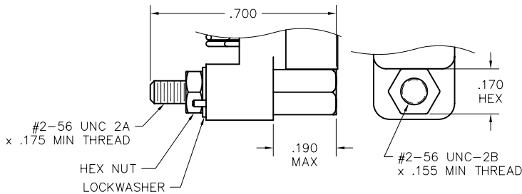
JACKPOST ASSEMBLY FACTORY INSTALLED ONLY
