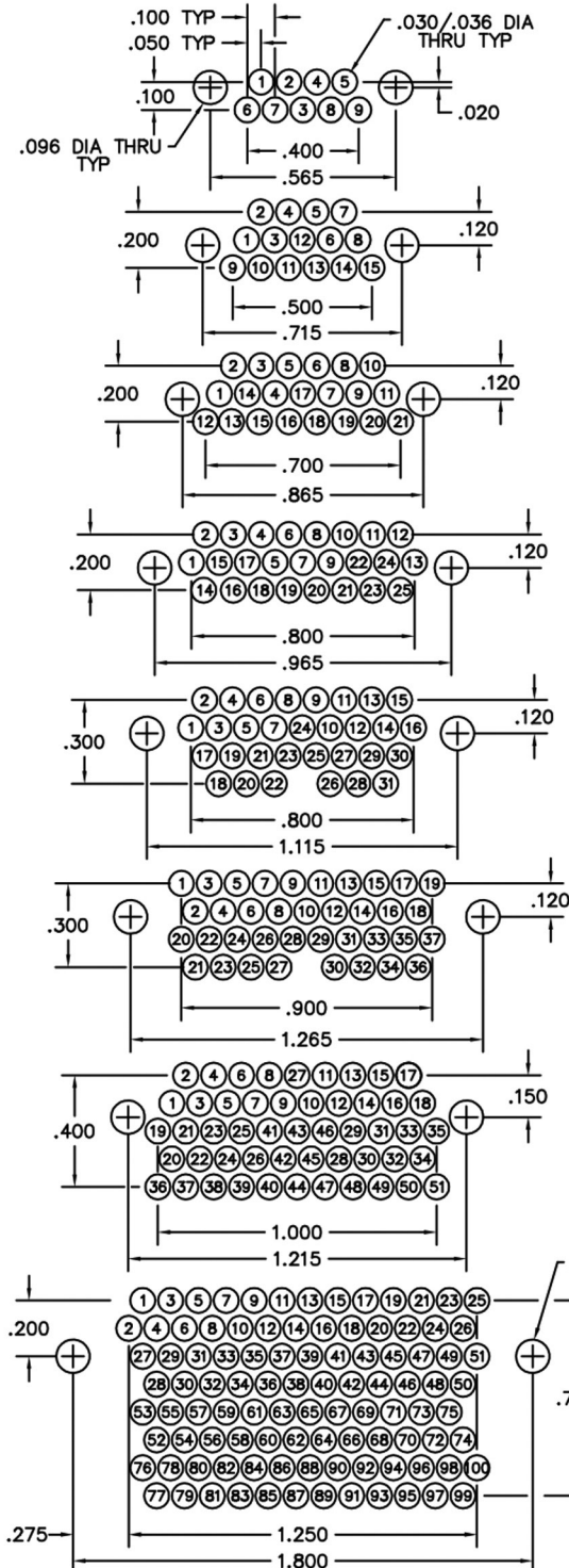
PLUG PC BOARD LAYOUT COMPONENT SIDE
