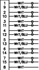
15 POSITION
