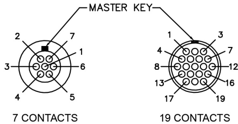
7 CONTACTS
