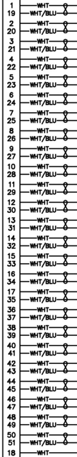
51 POSITION 3 rows
