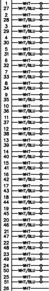
51 POSITION 2 rows
