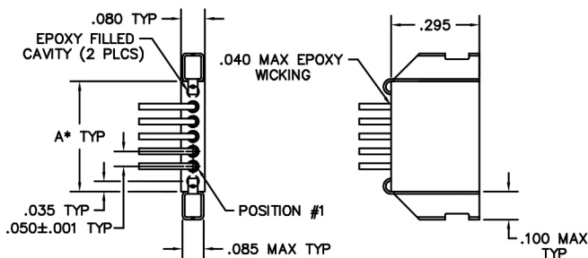
TERMINATION VIEW
