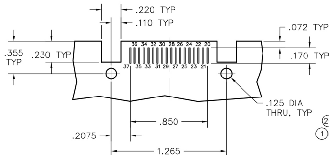
CONNECTOR MATING FACE
