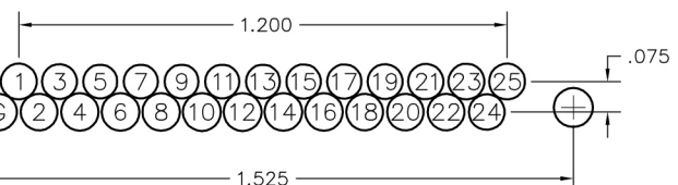
25 POSITION
