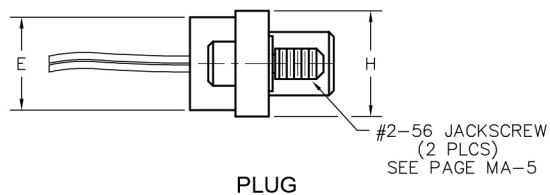
PLUG
