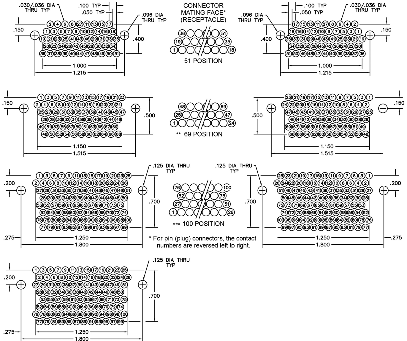
PLUG PC BOARD LAYOUT COMPONENT SIDE
