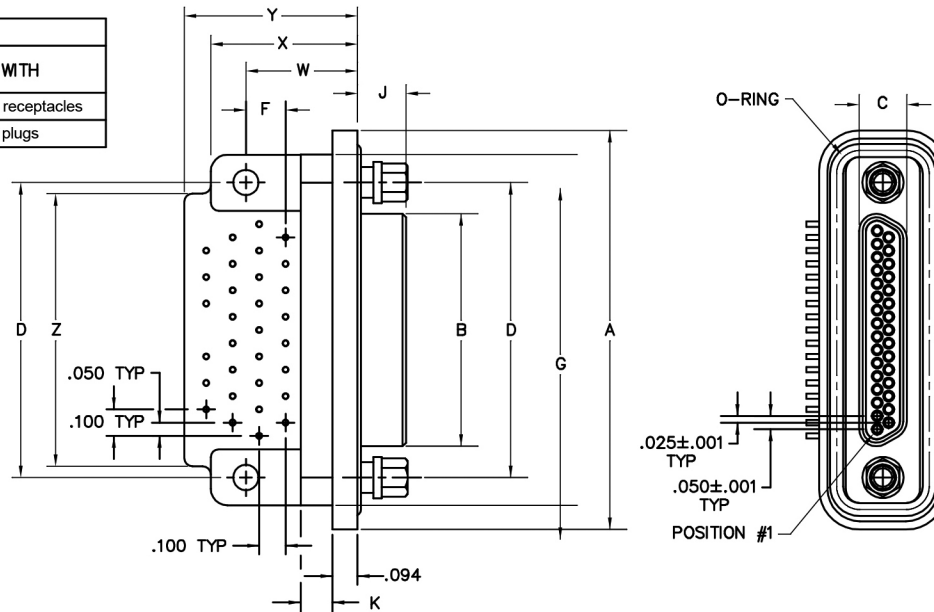
MK-2D2-031-335-260S (PLUG)
