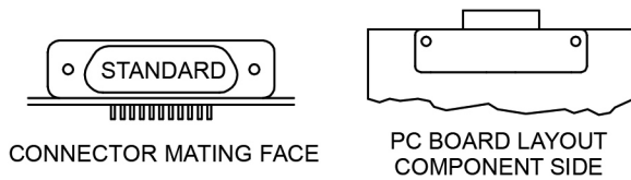
PLUG PC BOARD LAYOUT COMPONENT SIDE
