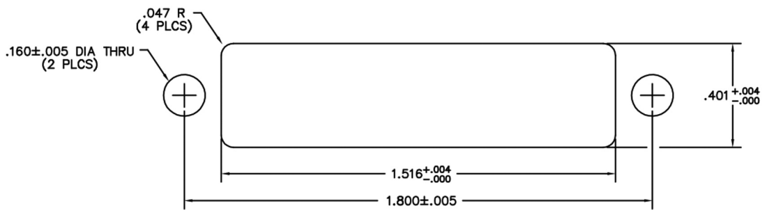
RUGGED METAL MM, MN, MK, ML SIZE 100
