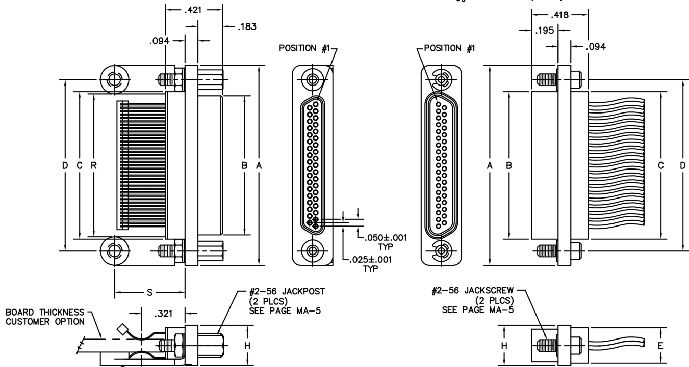
PLUG
