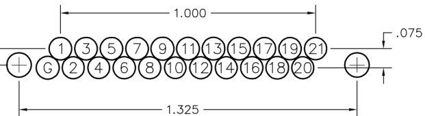
21 POSITION
