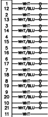
21 POSITION
