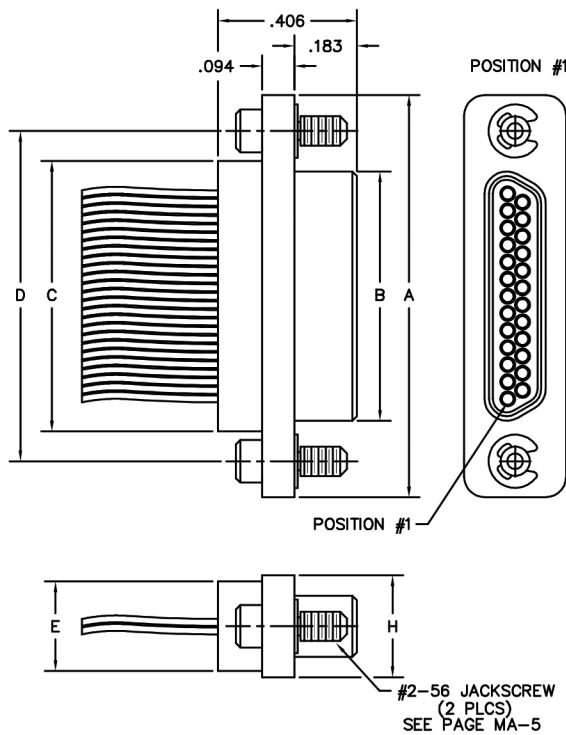
PLUG
