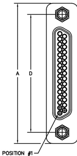
PLUG
