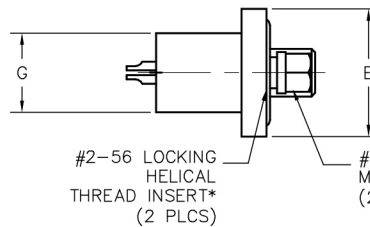
SOLDER CUP OR PIGTAIL TERMINATION (PLUG WITH SOLDER CUP TERMINATION SHOWN)
