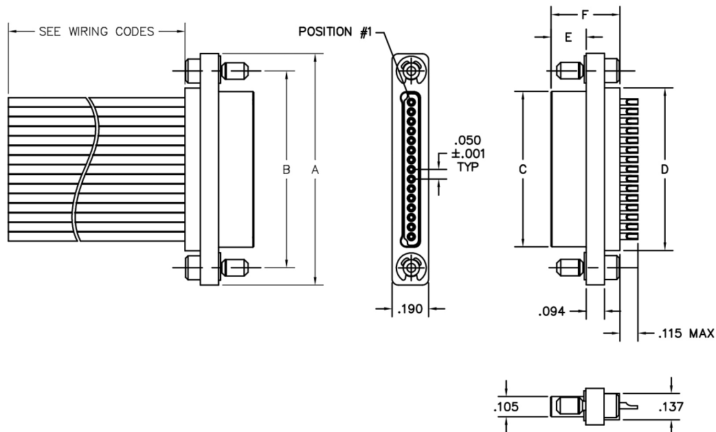
PLUG SHOWN
