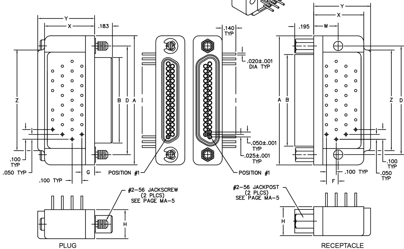
PLUG
