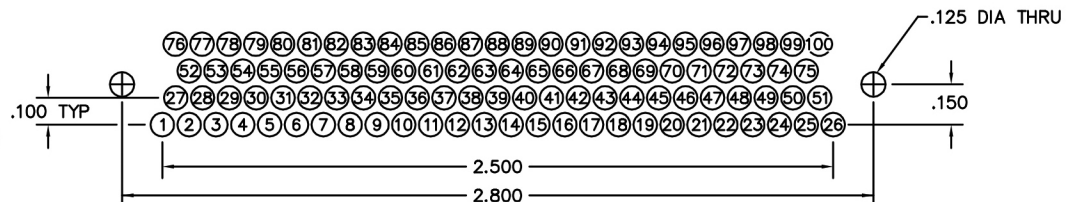
100 POSITION
