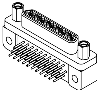
MK-2P2-031-A35-220S (PLUG)
