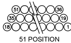
CONNECTOR MATING FACE (PLUG)
