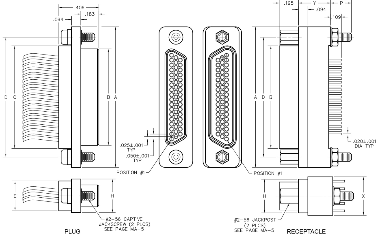
PLUG
