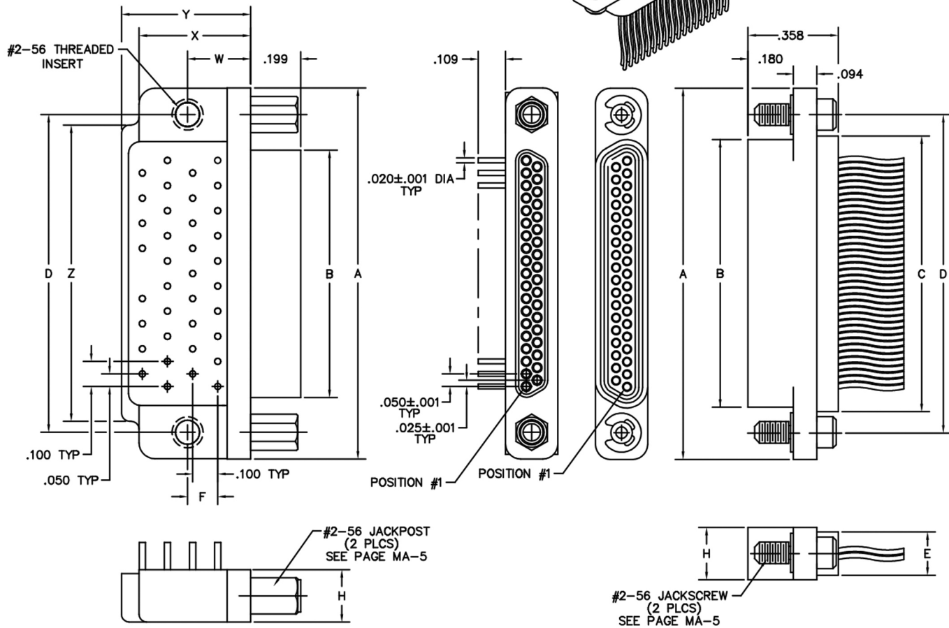
PLUG
