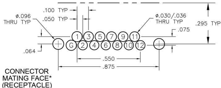
FRONT FACE OF FLANGE
