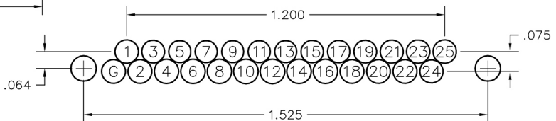
25 POSITION
