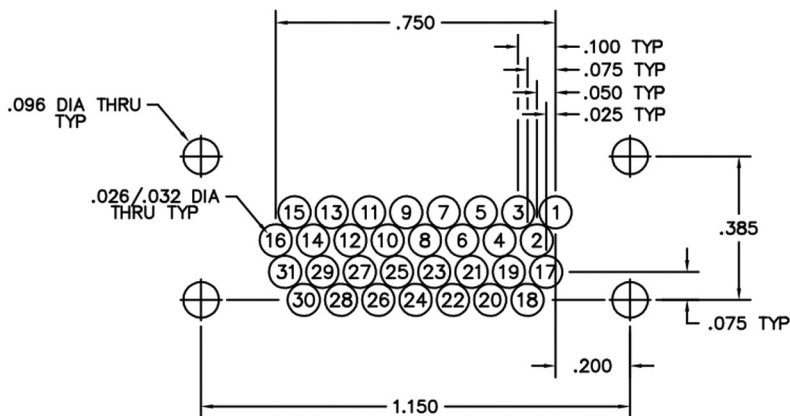
RECEPTACLE PC BOARD LAYOUT COMPONENT SIDE
