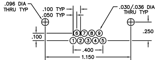
RECEPTACLE PC BOARD LAYOUT COMPONENT SIDE
