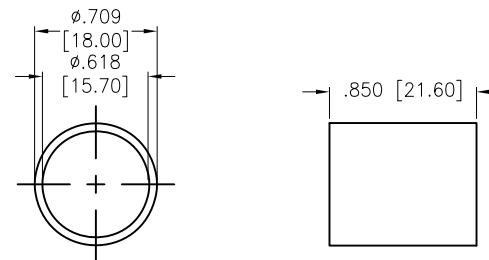
Plug Bushing For 2/0AWG&70mm 2 (250A) (Packaged separately in poly bag)
