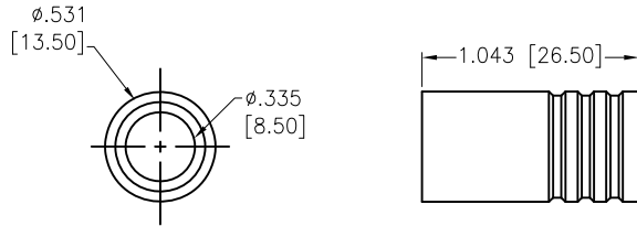
Seal Ring For 6AWG&16mm 2 (Packaged separately in poly bag)
