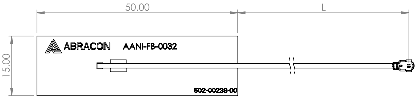
TOP VIEW
