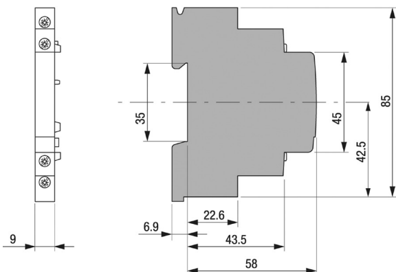
E299-11 AUXILIARY CONTACT
