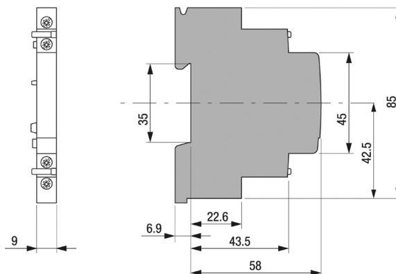
E299 AUXILIARY CONTACT
