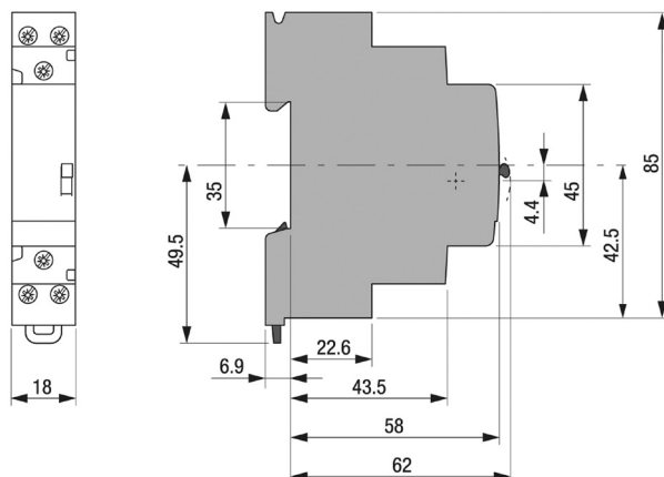
E297 INSTALLATION RELAY
