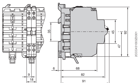
Auxiliary switch and signal contact
