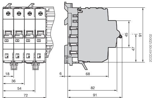
4-pole residual current operated circuit breaker, switch disconnector
