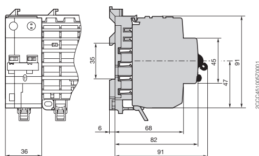
2-pole residual current operated circuit breaker F402
