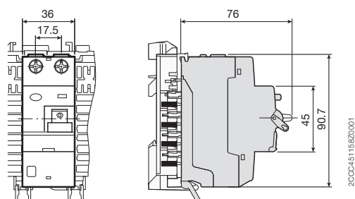
2-pole residual current operated circuit breaker F402
