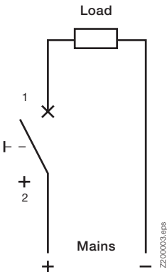
Connection diagram, single-pole (max. 220 V=) S401M-UCC
