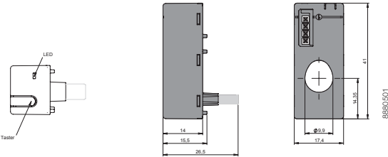
Universal adapter 32 A, 63 A
