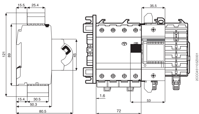
Residual current circuit-breakers with overcurrent protection (RCBO) FS401
