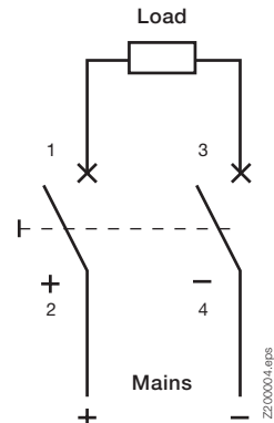
Connection diagram, two-pole (max. 440 V=) S402M-UCC
