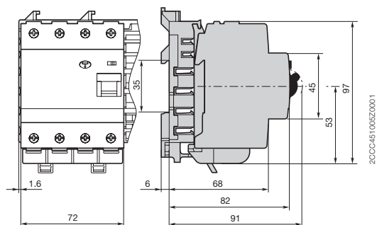
4-pole residual current operated circuit breaker, switch disconnector
