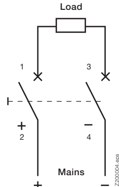
Connection diagram, two-pole (max. 440 V=) S402M-UCZ
