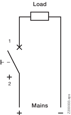
Connection diagram, single-pole (max. 220 V=) S401M-UCZ
