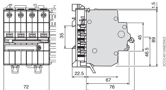
4-pole residual current operated circuit breaker
