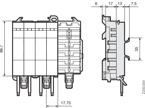
Universal adapter 32 A, 63 A
