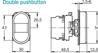
Double pushbutton
