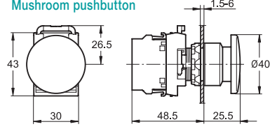
Mushroom pushbutton
