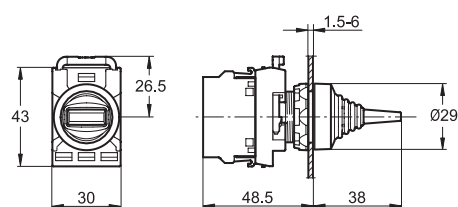
Toggle switch
