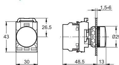
Pilot light
