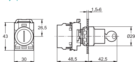
Key-operated selector switch
