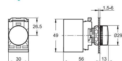
Pilot light with transformer
