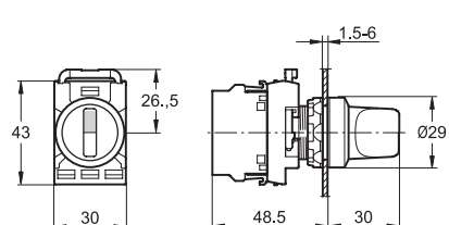
Selector switch
