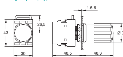
Emergency stop type MPE
