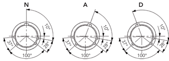
Viewed from front face of plug
