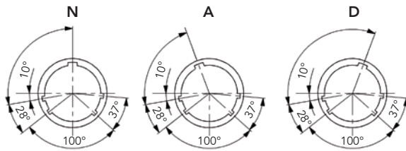
Viewed from front face of receptacle
