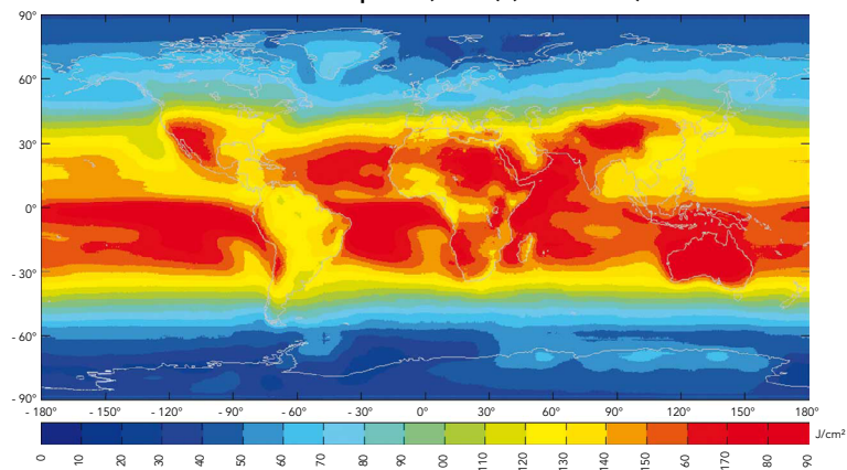
Yearly mean of daily irradiation in UV (280-400 nm) on horizontal plane ( \text{J}/\text{cm}^2 ) (1990-2004)
