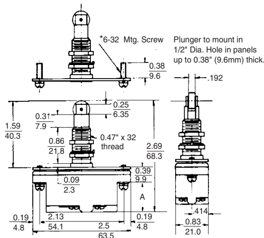
Type AP301, 303, 304, 305, 321, 323, 324, 325, and CP321, 323, 324, 325
