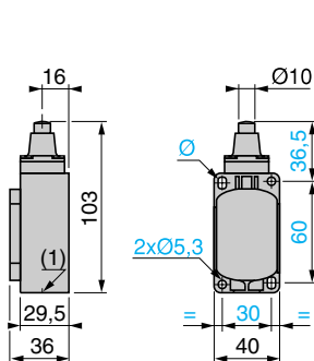
XCKS•39 ZCKS• + ZCKD39
