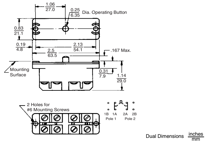
Class 9007 Type CO, Two-Pole Snap Switch
