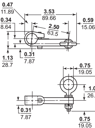
Cable Operated Type B27
