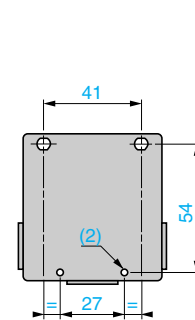
Rear view XCKM•••, ZCKM•, ZCKMD3•
