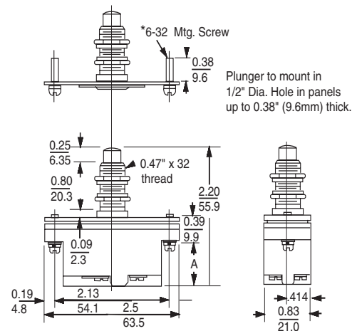
Type AP201, 221, and CP221
