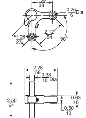
Cable Operated with Reset Type Y3
