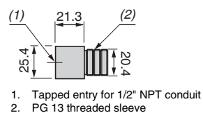
DE9RA1212 (PG 13 to 1/2" NPT adapter)
