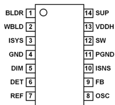
Figure 2. Pin configuration
