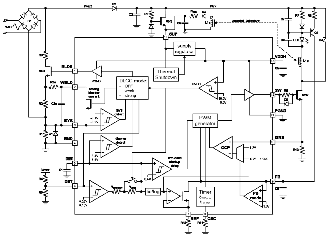
Figure 4. Block diagram
