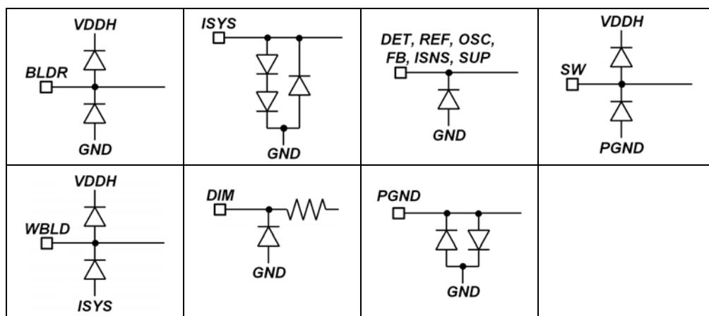
Figure 3. Equivalent circuit
