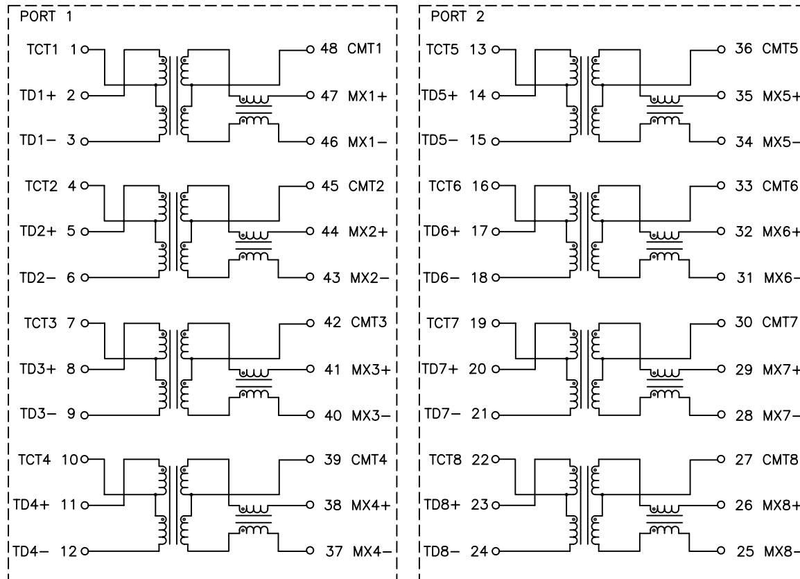
SCHEMATIC
