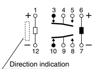
Schematic (Bottom view) 2 coil latching
